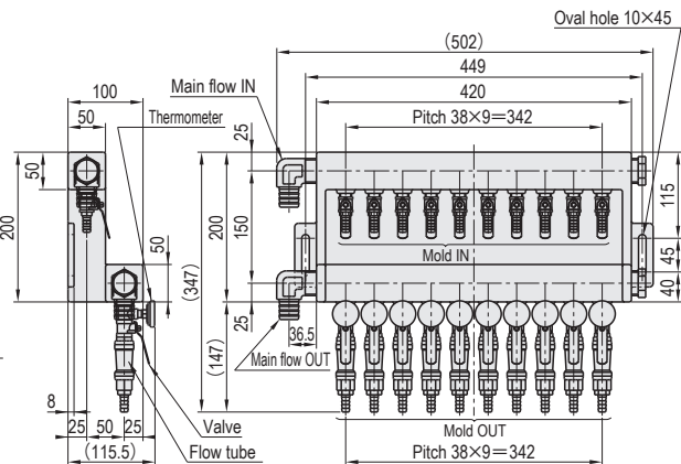
M-CMF-B-10-10
