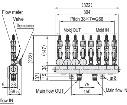
M-CMF-B-4-4
