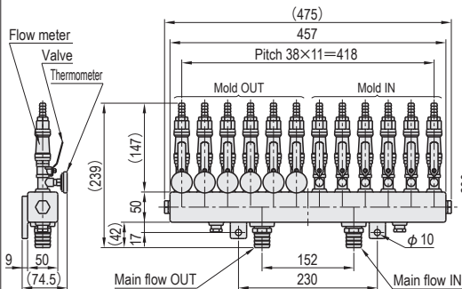
M-CMF-B-6-6
