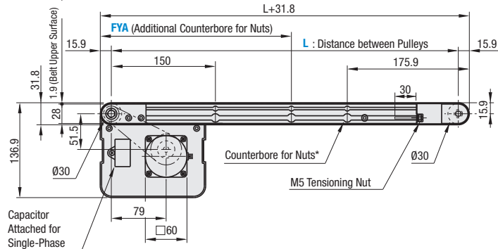
25W Motor Type
