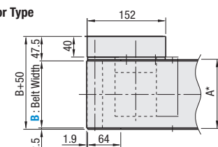
25W Motor Type
