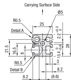
Frame Cross Section and Enlarged View (Symmetrical)
