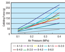
SKNS Air Colliding Force Property Table
