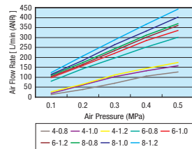
SKNF Air Flow Rate Property Table
